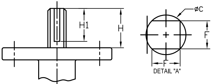
ASSOCIATED VALVE DETAIL (FNW 7xx-Series Resilient seat BFVs)
